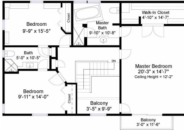
Second Floor Plan Ceiling Height = 8'-0"
